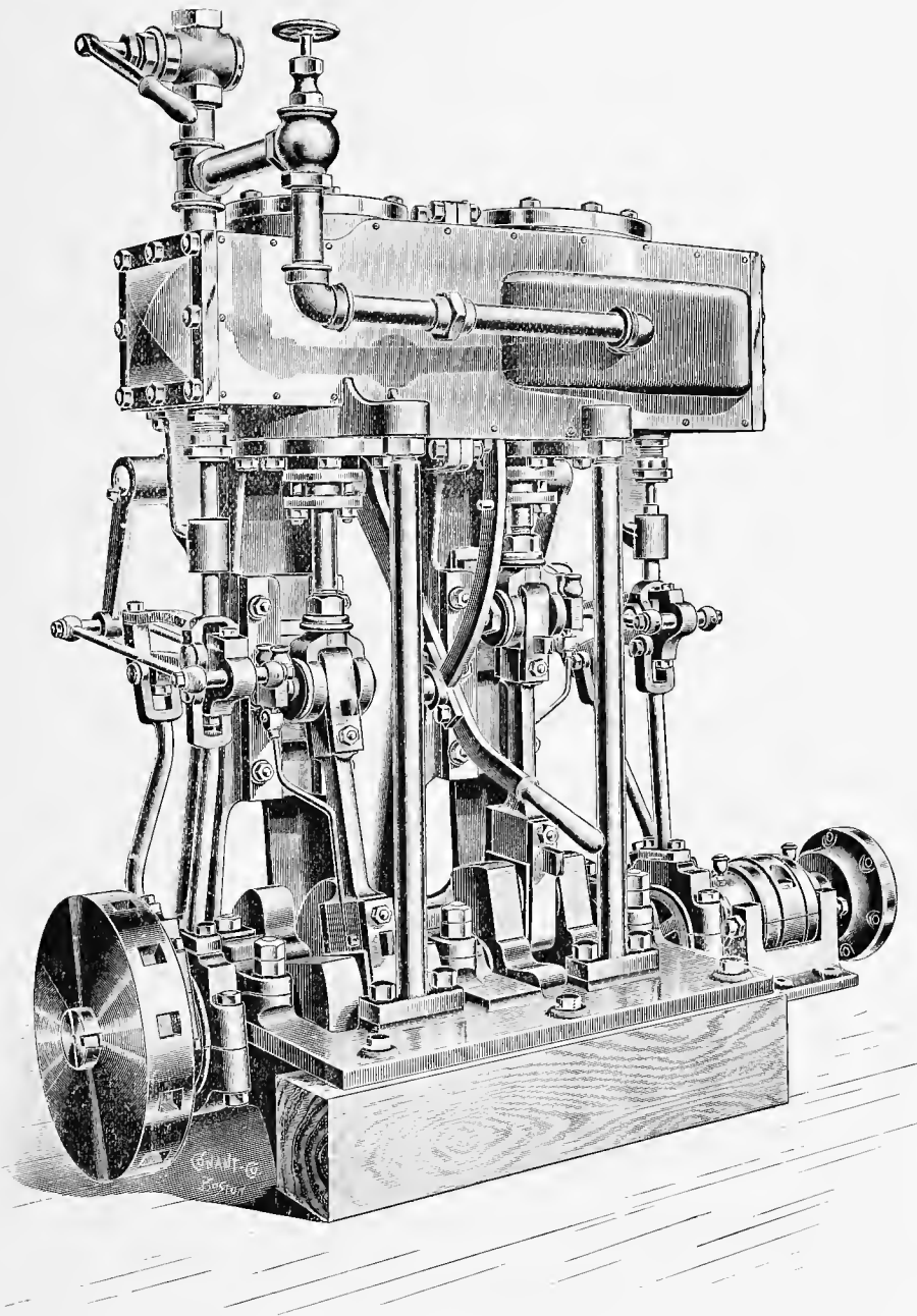
THE MORRIS COMPOUND MARINE ENGINE.—Built by the Morris Machine Works.
